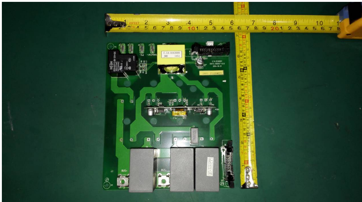
Photo 20 Boost board front view
