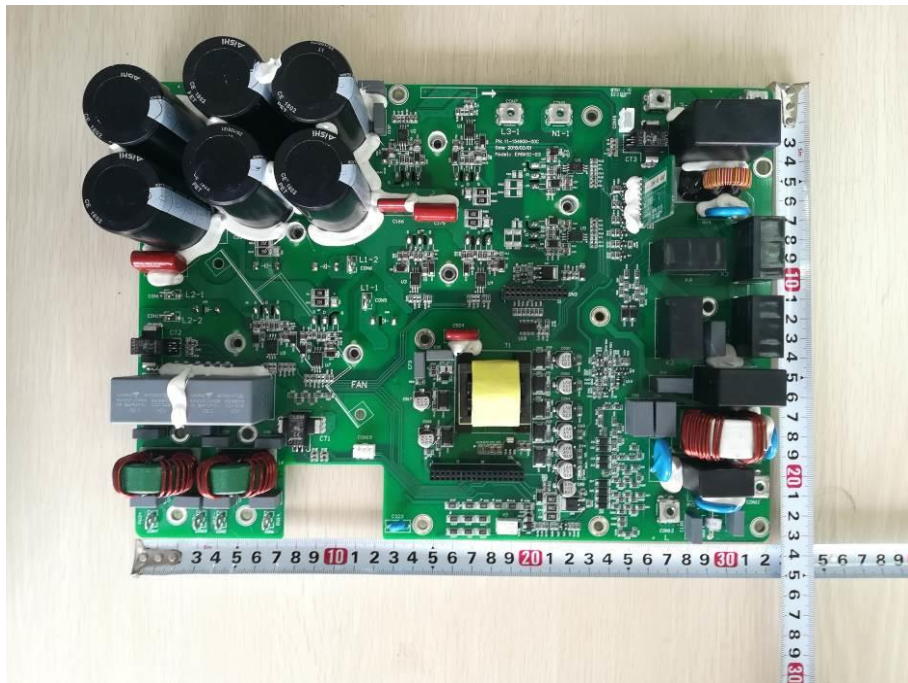
Figura 5. Vista lado dos componentes da placa principal Figure 5. Component side view of Main board
