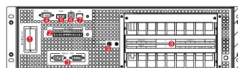
20-30kVA Rear Panel
