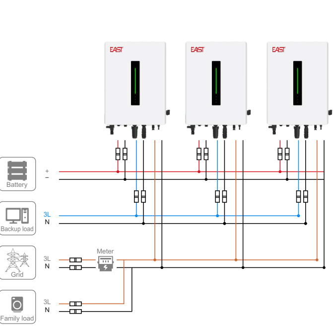
Parallel application
