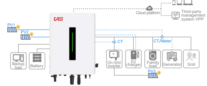
Typical application 2
