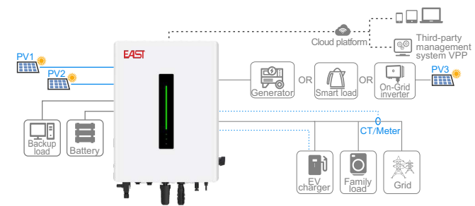
Typical application 1
