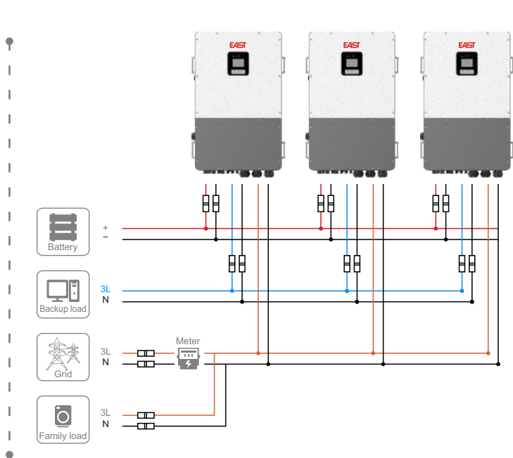
Parallel application
