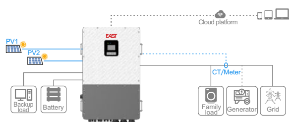
Typical application 2
